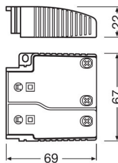
OT CABLE CLAMP B-STYLE LP
