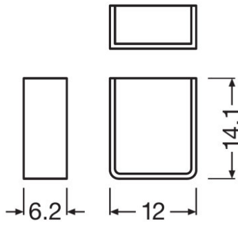
728405_Single sided endcaps for side-bending modules
