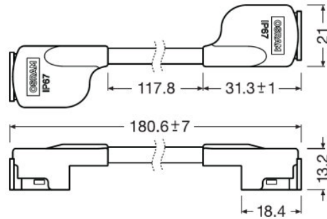
JUMPER-FLEX-IP67-2P
