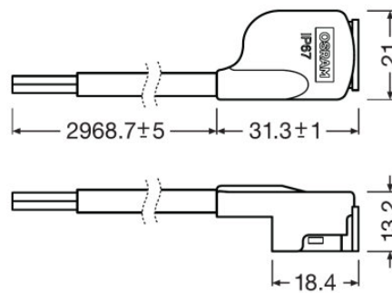
CONN-FLEX-IP67-2P-300
