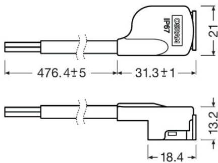
CONN-FLEX-IP67-2P
